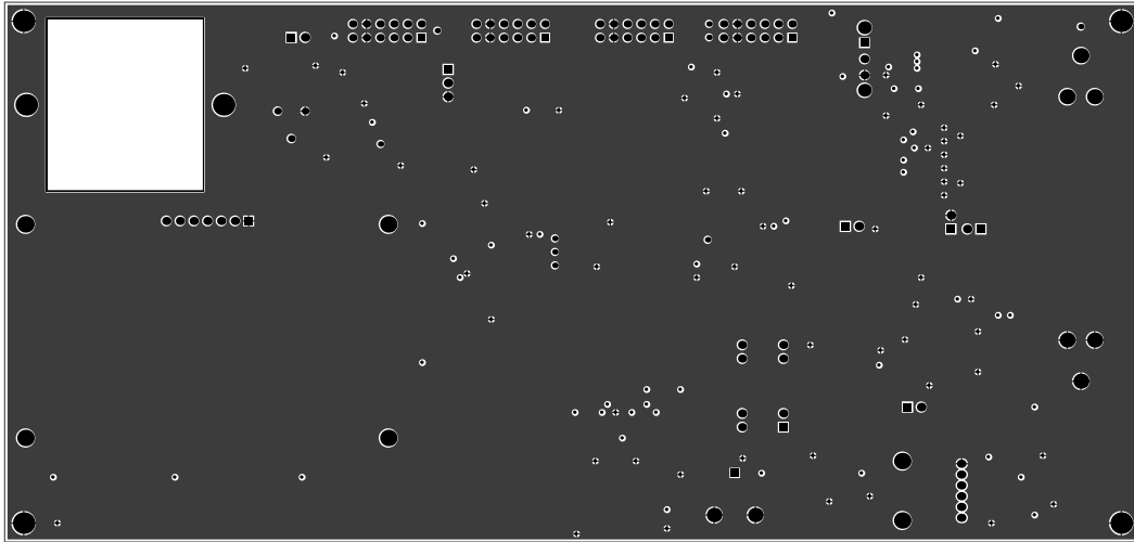
SIGNAL LAYER 1 BOARD OUTLINE
