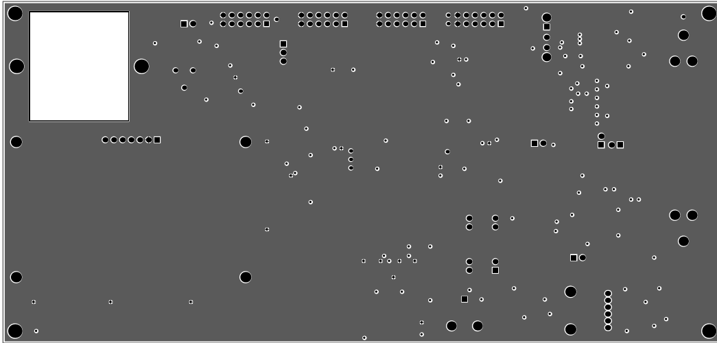
SIGNAL LAYER 2 BOARD OUTLINE
